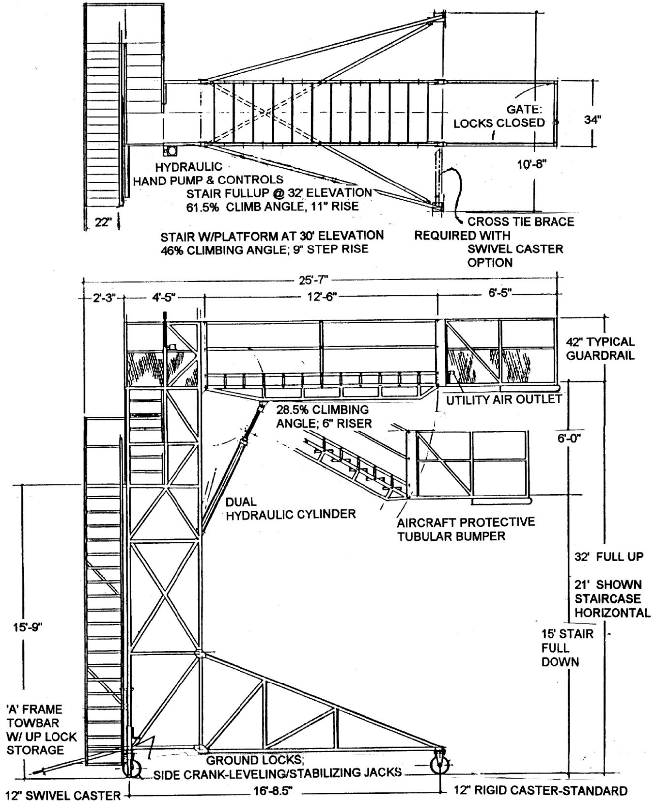
MODEL 3483 HIGH REACH ADJUSTABLE SERVICE & WORKSTAND 17 FT ADJUSTMENT RANGE FROM 15 FEET TO 32 FEET
